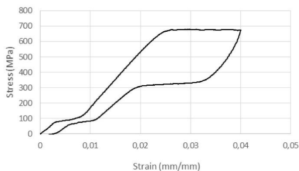
Figure 7 Typical hysteresis behaviour of 0.25 mm Nitinol wire bundles.
