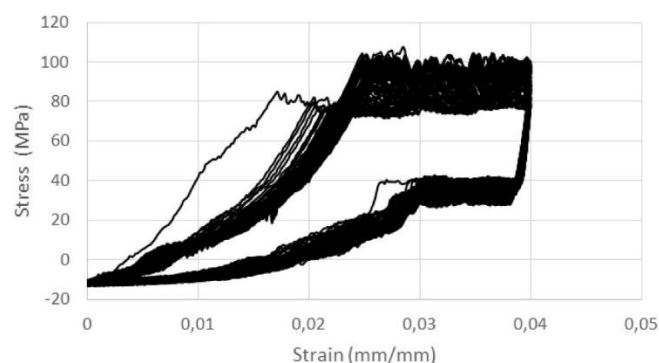
Figure 8 Typical cyclic-dynamic testing of 0.25 mm Nitinol wire Bundles (4% strain).
