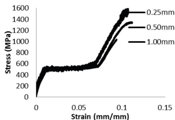
Figure 6 Stress vs. strain (tensile testing of single wires).
