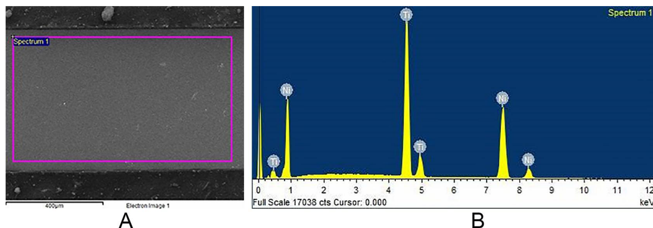
Figure 4 (a) EM Image of the bulk area of 1 mm diameter Nitinol wire section; (b) DX elemental analysis of 1 mm diameter Nitinol wire.
