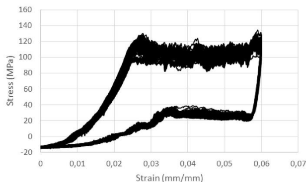
Figure 9 Typical cyclic-dynamic testing of 0.25 mm Nitinol wire bundles (6% strain).
