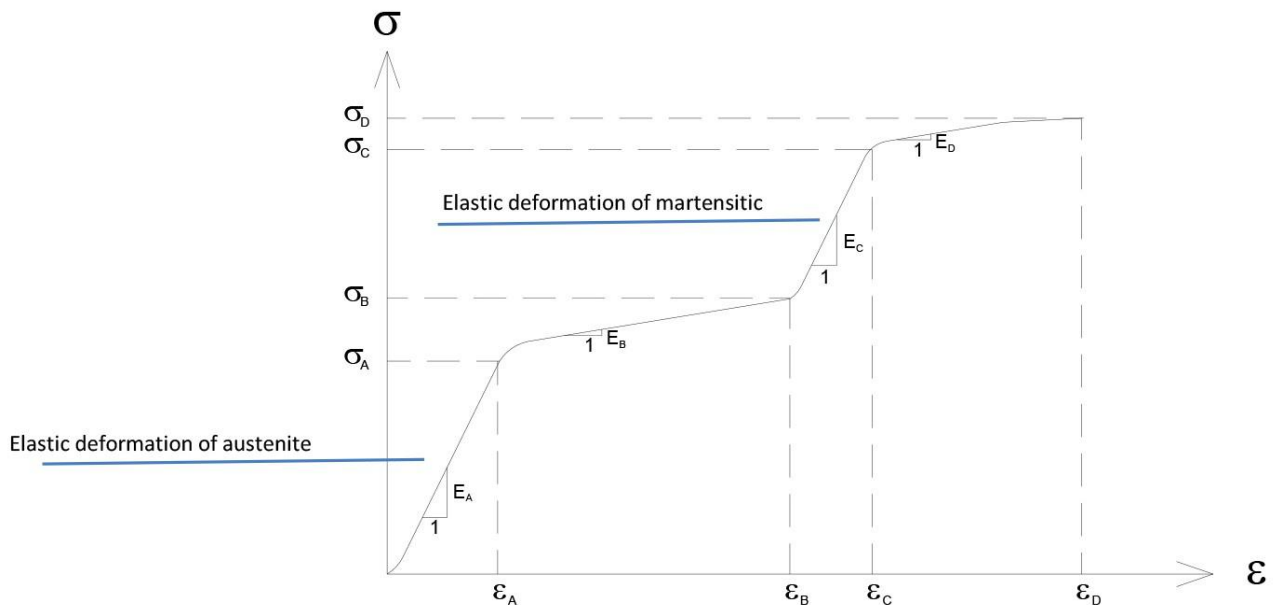
Figure 2 Stress-strain diagram of Nitinol. \sigma_A and \sigma_B are the critical stresses at which martensitic transformation starts and finishes [34].
