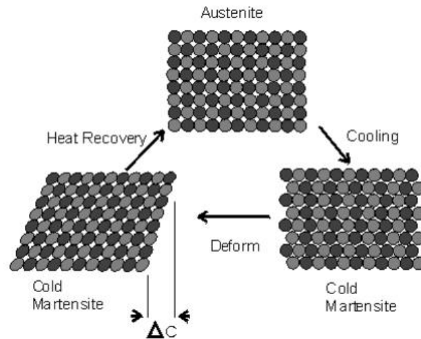
Figure 1 Phase transformations of Nitinol [33].
