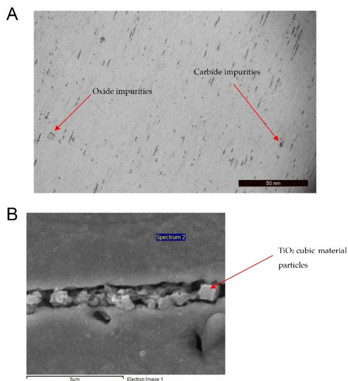
Figure 5 (a) The optical microscope image of the etched 1.0 mm diameter Nitinol wire; (b) electron Microscope Image of particles in the stringer of 0.5 mm diameter Nitinol wire.
