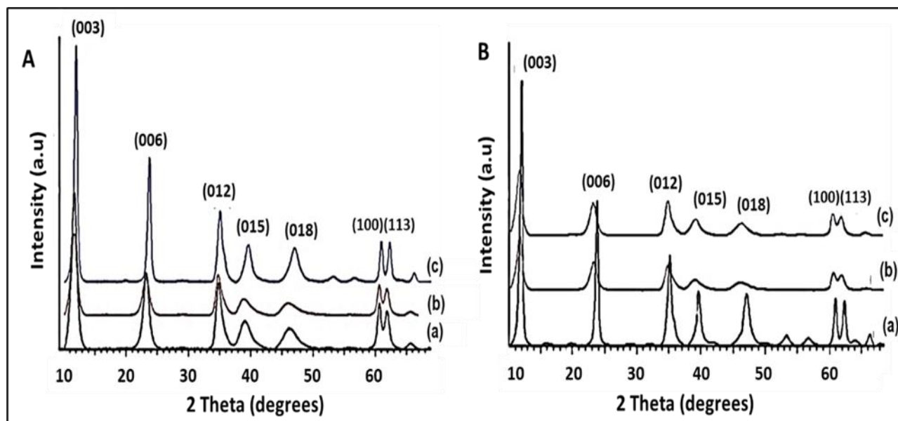
Figure S1 The XRD diffractograms of A: MgAlArg 0.25 (a), MgAlHist 0.25(b), MgAl 0.25 (c); and (B) MgAl 0.33 (a), (MgAlArg 0.33 (b), MgAlHist 0.33 (c).
