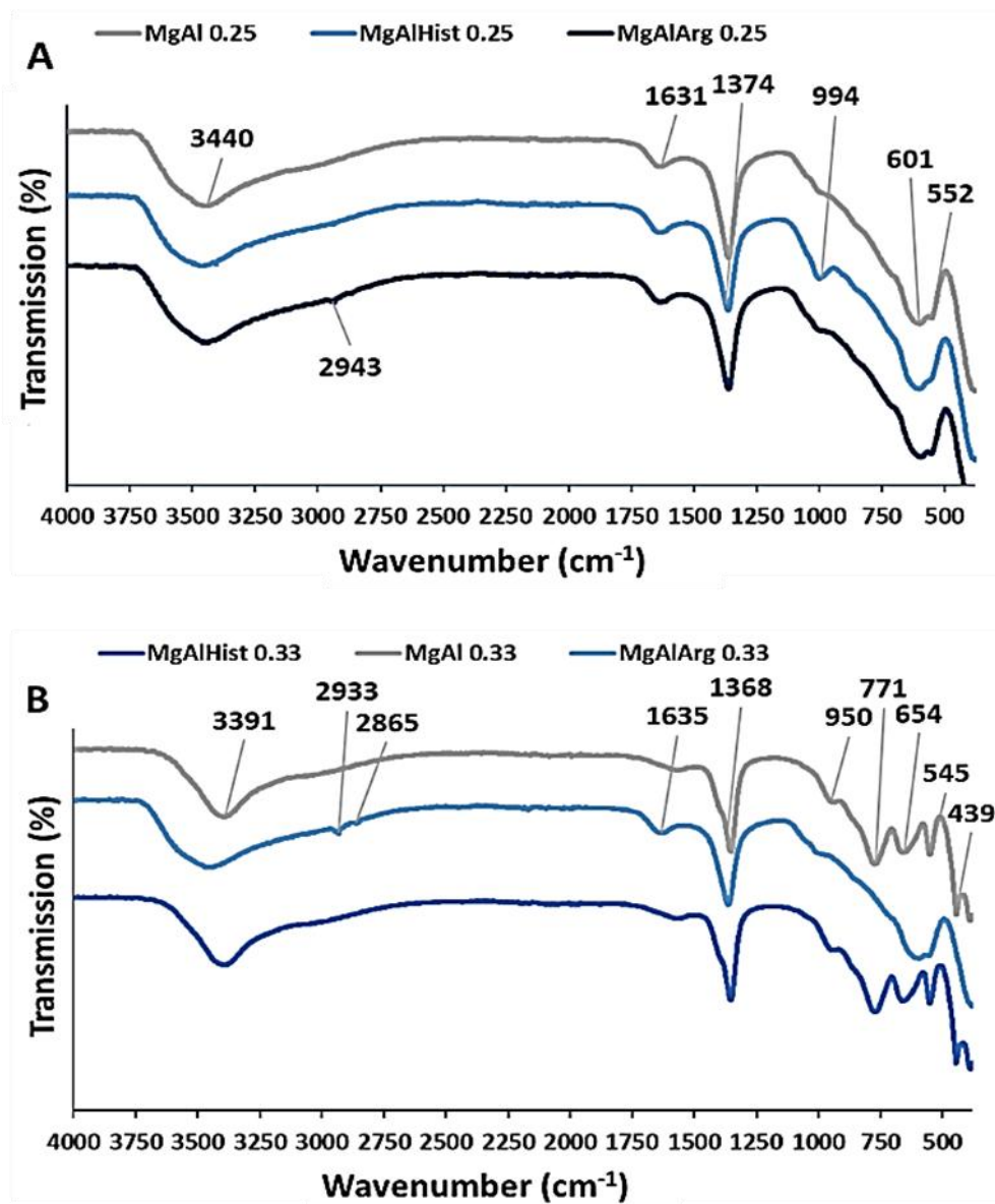
Figure S2 FTIR spectra of (A) MgAl 0.25, MgAlArg 0.25 and MgAlHist 0.25; and (B) MgAl0.33, MgAlArg 0.33 and MgAlHist 0.33.
