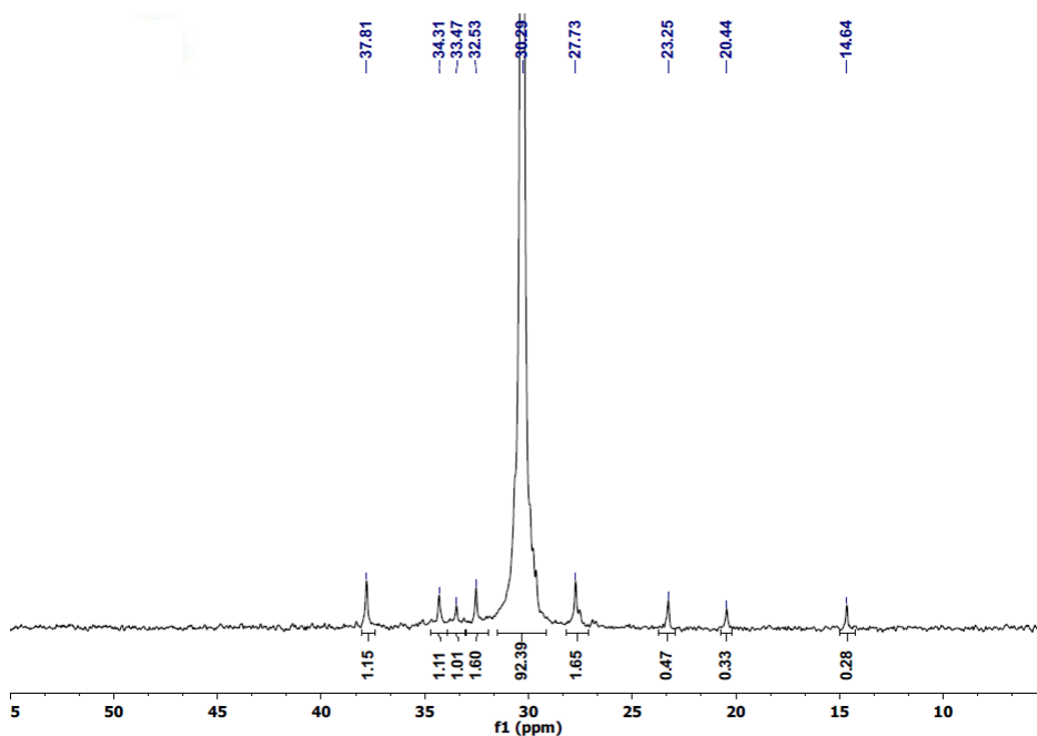
Figure S6 13 C-NMR spectrum of PE-C170.
