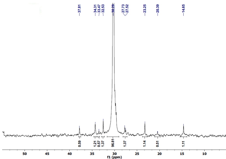
Figure S4 ^{13}\text{C} -NMR spectrum of PE-C125.
