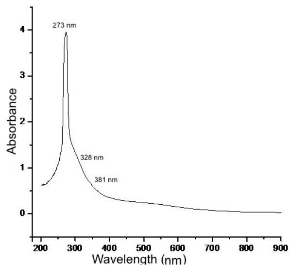
Figure S2 UV-Vis absorbance spectrum of the C1 complex.
