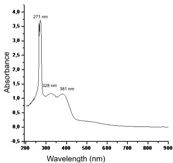
Figure S1 UV-Vis absorbance spectrum of the N1C2 complex.
