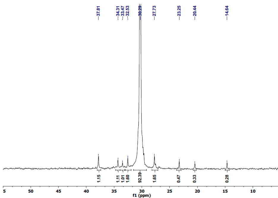
Figure S5 13 C-NMR spectrum of PE-C150.
