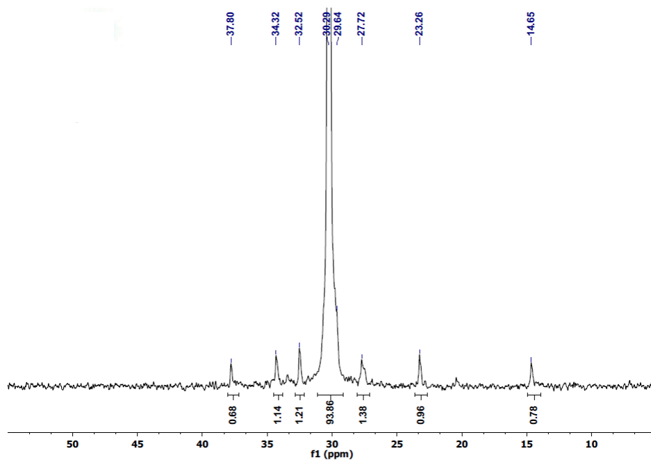
Figure S3 ^{13}\text{C} -NMR spectrum of PE-N1C1.
