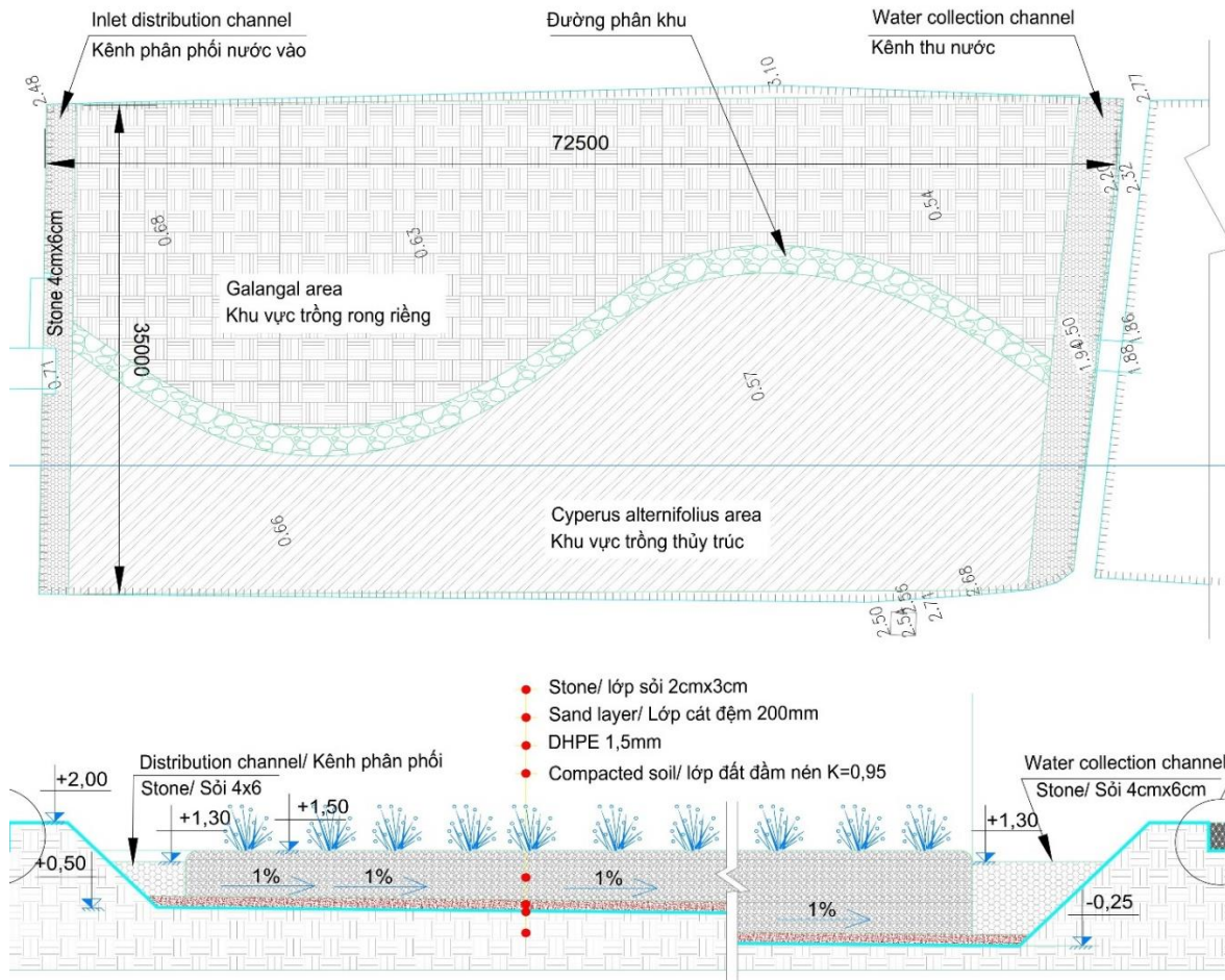
Figure S4 Diagram of the constructed wetland.
