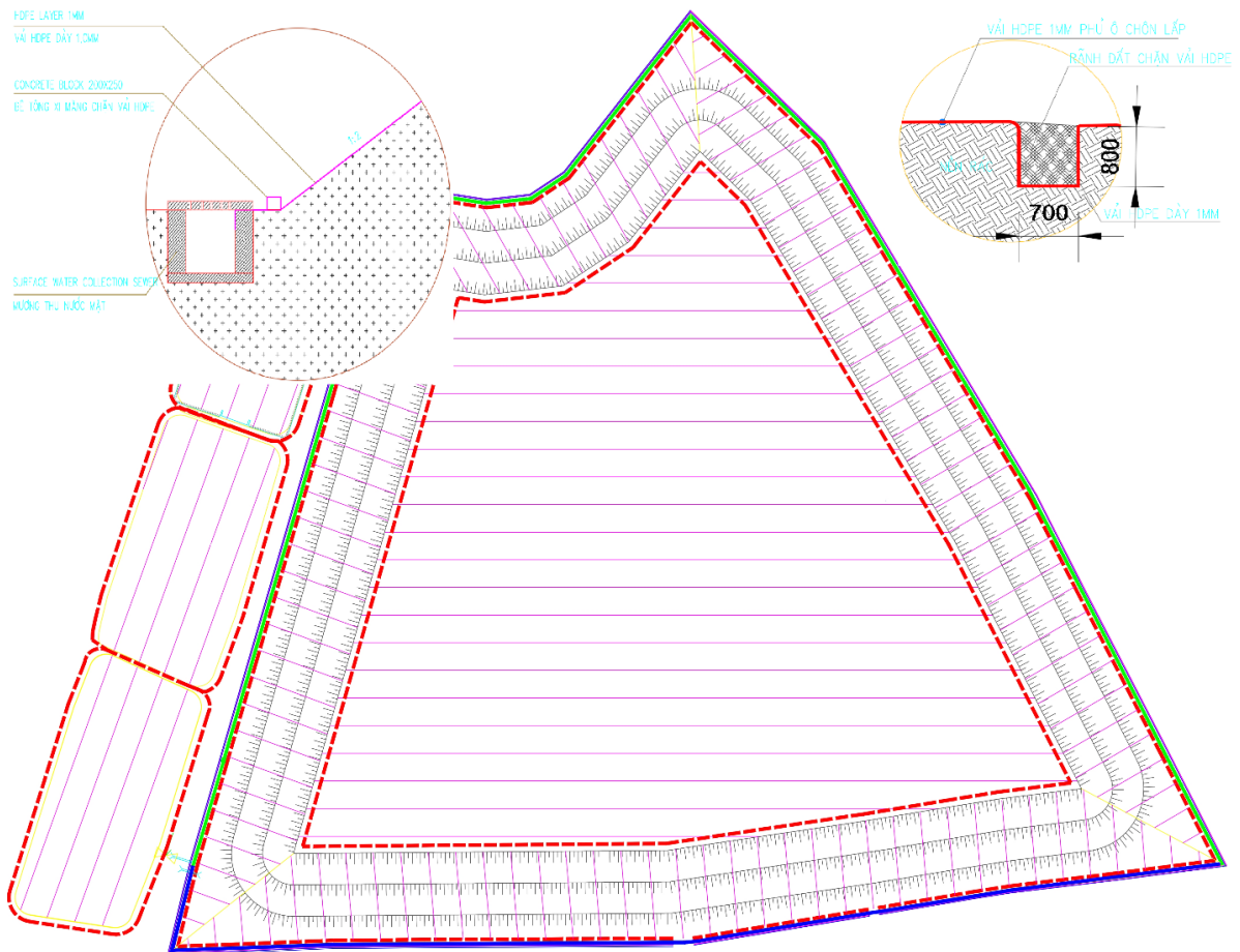
Figure S2 Geotextile spreading and anchoring outline.
