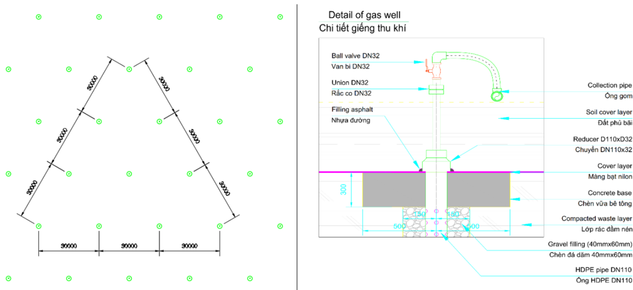
Figure S5 Structure and arrangement of gas collection pipes.
