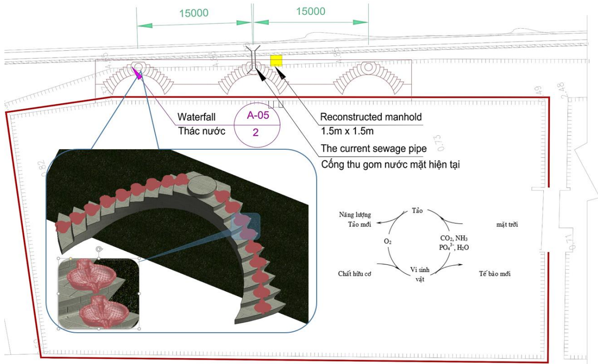
Figure S3 Layout of aeration waterfalls in a flow-directing aerated system.
