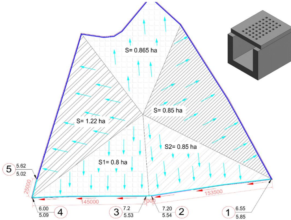
Figure S1 Drainage zoning and sewer structure.
